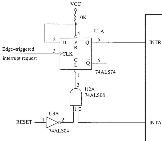
FIGURE 12-11 Converting INTR into an edge-triggered interrupt request input.
